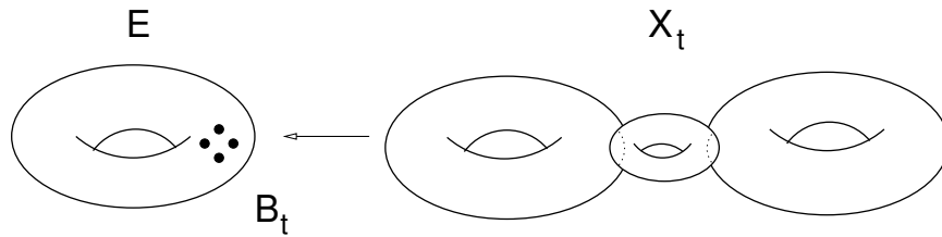
Figure 5. A degree two branched cover.
