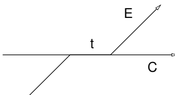
Figure 3. A right twist on C adds t to the period of E .
