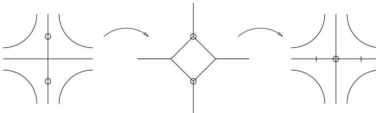
Figure 4. Folding at a zero of \omega .
