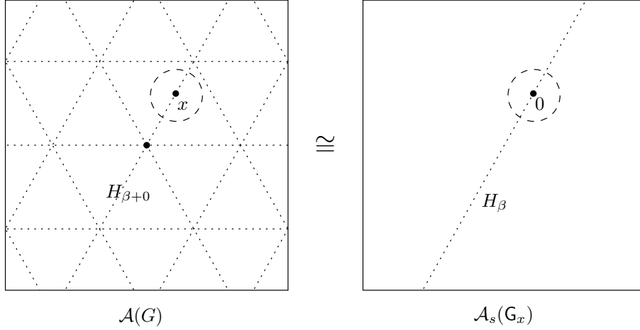
Figure 3.2: The affine apartment of SL_3(k) , as compared to the spherical apartment of G_x , which is isomorphic to GL_2(f) .
