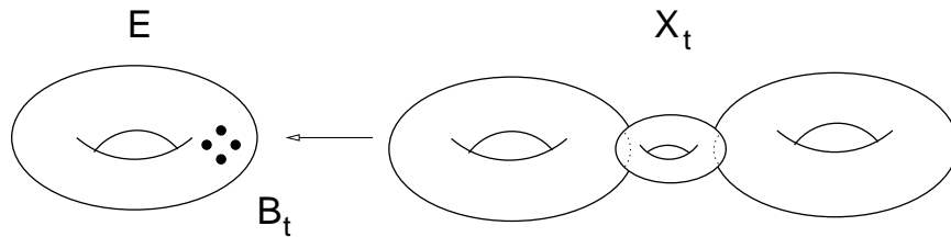
Figure 5. A degree two branched cover.
