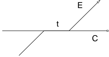
Figure 3. A right twist on C adds t to the period of E .
