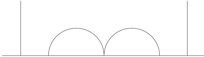
Figure 4. A fundamental domain for G_0 .
