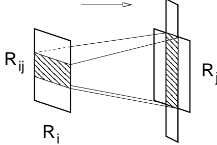
Figure 1. Geodesic flow on a Markov section.
