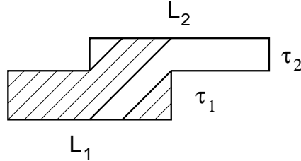
Figure 8. Splitting for t = \tau_1 + \tau_2 .
