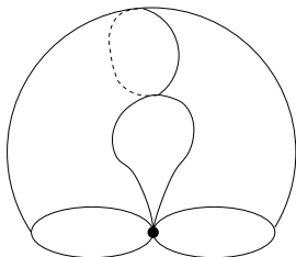
Figure 4. A cylinder with two boundary points identified at a zero of \rho .
