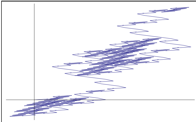
Figure 5. Zero flux leaves for cubic fields.
